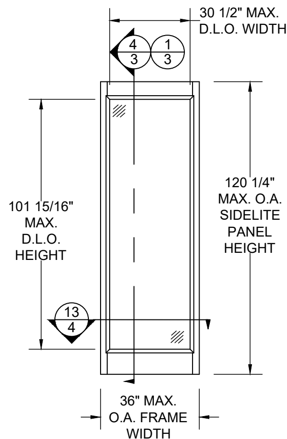
GLAZED SASH SET PANEL (SIDELITE & TRANSOM PANELS)
