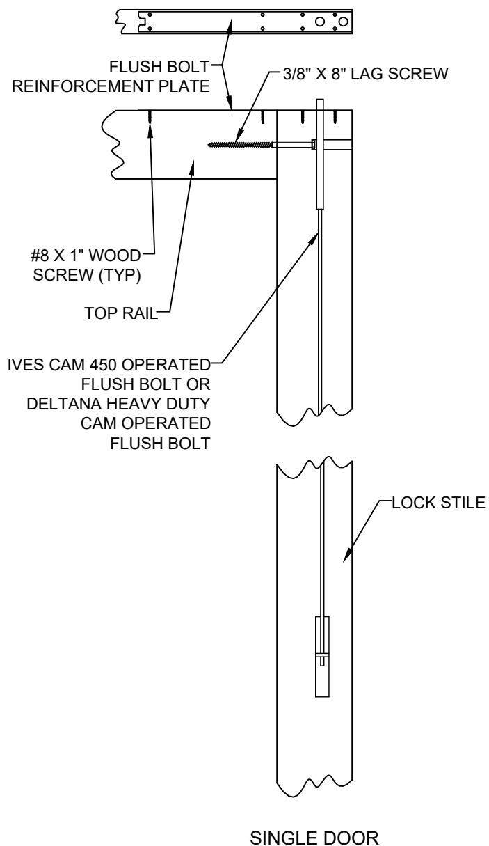
FLUSH BOLT DETAIL
