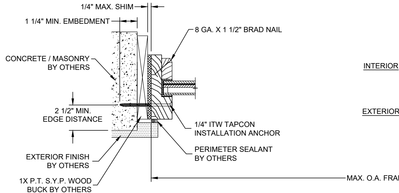
Y HORIZONTAL SECTION GLAZED SIDELITE/ TRANSOM PANEL AT JAMB CONCRETE / MASONRY SUBSTRATE OUTSWING SHOWN / INSWING OPPOSITE (SEE SHEET 4 SECTION 14 FOR APPROPRIATE SIDELITE & TRANSOM PANELS)
