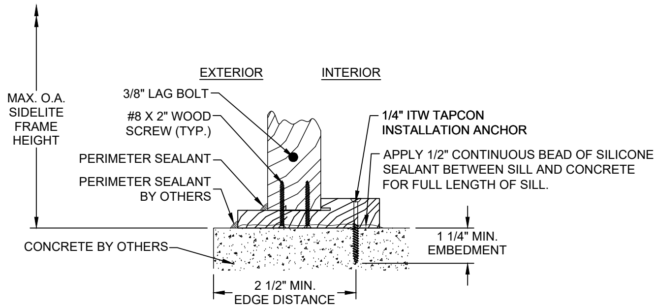
Q VERTICAL SECTION GLAZED SIDELITE PANEL AT SILL CONCRETE / MASONRY SUBSTRATE OUTSWING SHOWN / INSWING OPPOSITE (SEE SHEET 3 SECTIONS 1, 2, 3, 4 & 6 FOR APPROPRIATE SIDELITE PANELS)
