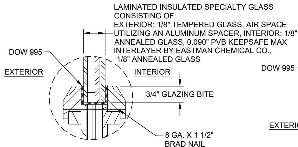
GLAZING DETAIL 3
