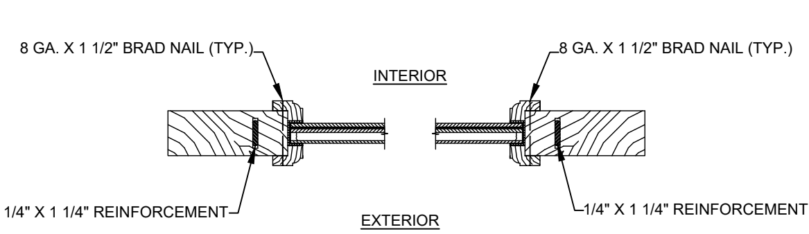
10 4 HORIZONTAL CROSS SECTION 2 1/4" FULL LITE DOOR & GLAZED 3/4 LITE OVER 2 1/4" WOOD DOOR PANEL & OPTIONAL SIDELITE PANELS
