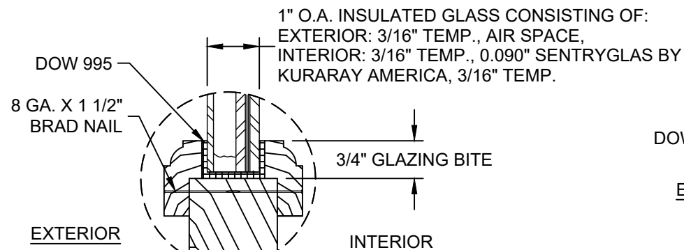
GLAZING DETAIL 1
