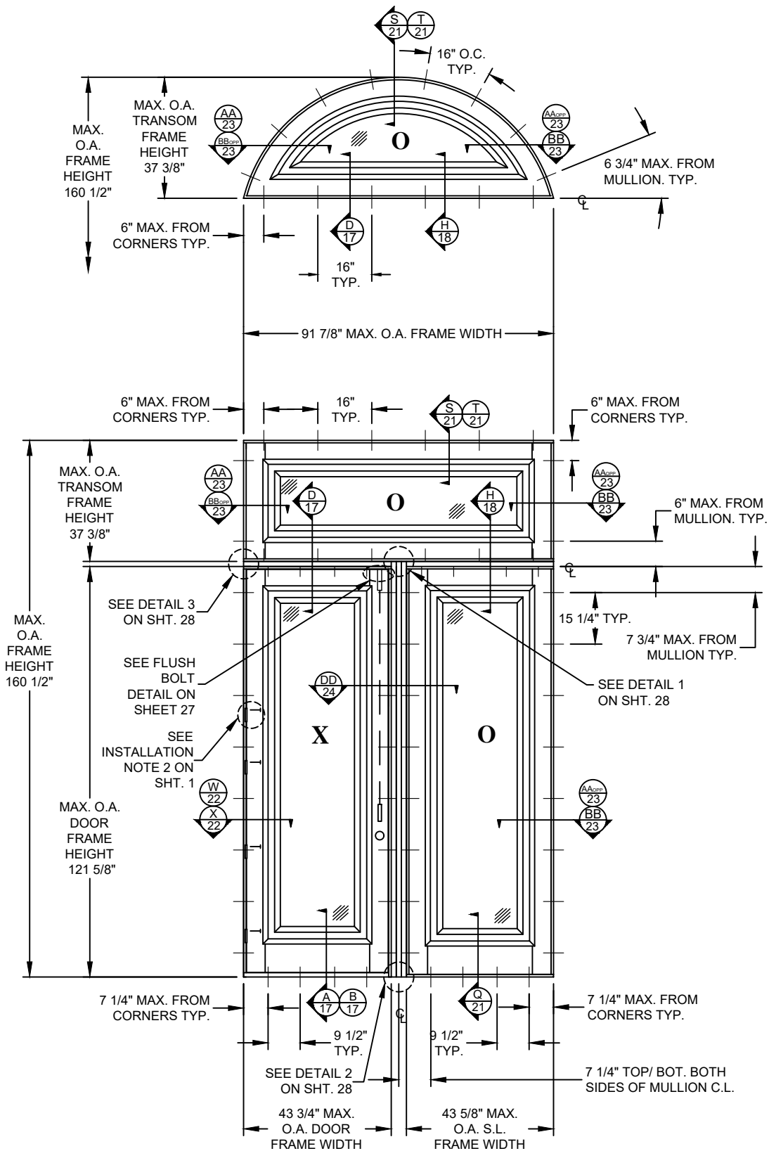
ELEVATION & ANCHOR LAYOUT GLAZED/OPAQUE SINGLE DOOR W/ GLAZED PANEL INSERT SIDELITE & GLAZED PANEL INSERT SQUARE/RADIUS TOP TRANSOM INSWING / OUTSWING EXTERIOR VIEW
