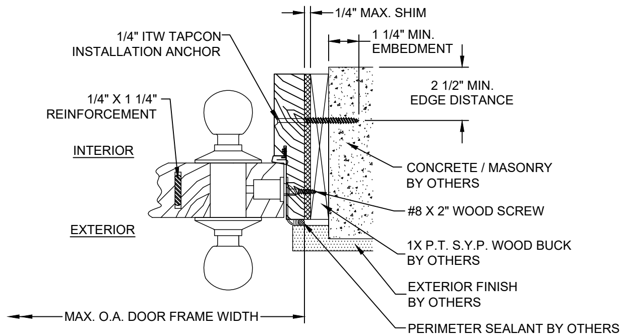
U HORIZONTAL SECTION GLAZED/OPAQUE DOOR PANEL AT LOCK STILE CONCRETE / MASONRY SUBSTRATE OUTSWING SHOWN / INSWING OPPOSITE (SEE SHEET 4 SECTIONS 10, 11 & 12 FOR APPROPRIATE DOOR PANELS)
