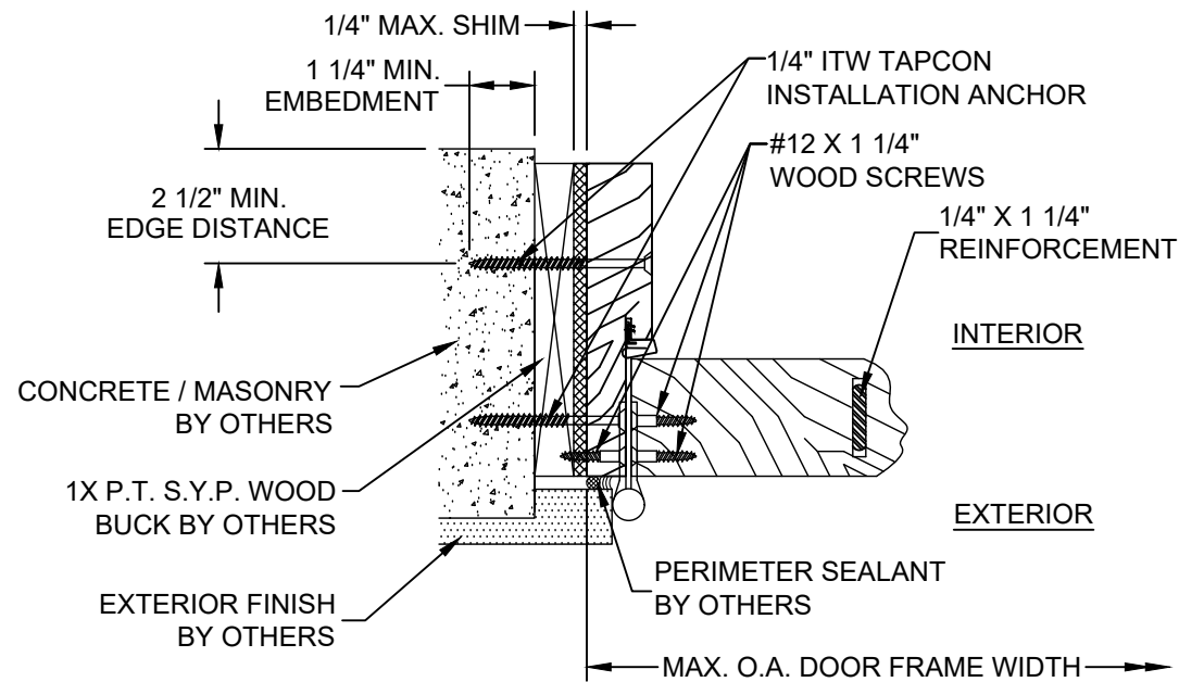
W HORIZONTAL SECTION GLAZED/OPAQUE DOOR PANEL AT HINGED JAMB CONCRETE / MASONRY SUBSTRATE OUTSWING SHOWN / INSWING OPPOSITE (SEE SHEET 4 SECTIONS 10, 11 & 12 FOR APPROPRIATE DOOR PANELS)
