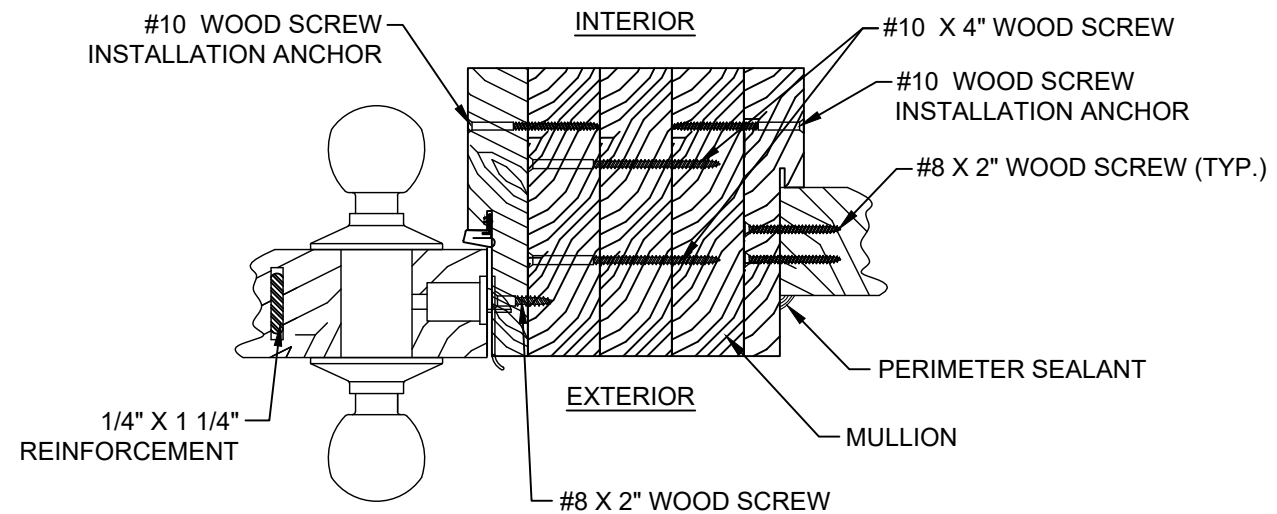
II HORIZONTAL SECTION GLAZED/OPAQUE DOOR PANEL W/ GLAZED/OPAQUE SIDELITE PANEL AT MULLION OUTSWING SHOWN / INSWING OPPOSITE (SEE SHEET 4 SECTIONS 10, 11 & 12 FOR APPROPRIATE DOOR PANELS & SHEET 4 SECTION 13 & 15 FOR APPROPRIATE SIDELITE PANELS)
