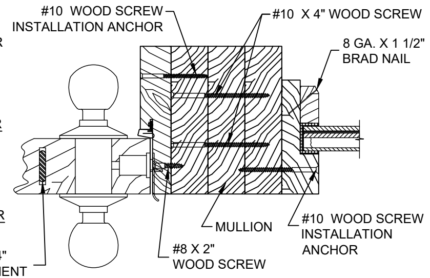
LL HORIZONTAL SECTION GLAZED/OPAQUE DOOR PANEL W/ GLAZED SIDELITE PANEL AT MULLION OUTSWING SHOWN / INSWING OPPOSITE (SEE SHEET 4 SECTIONS 10, 11 & 12 FOR APPROPRIATE DOOR PANELS & SHEET 4 SECTION 14 FOR APPROPRIATE SIDELITE PANEL)
