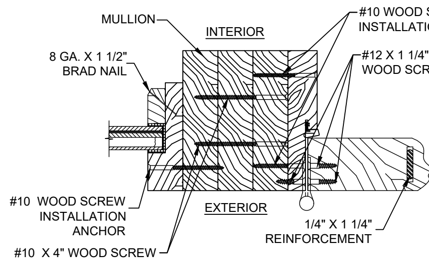
JJ HORIZONTAL SECTION GLAZED SIDELITE PANEL JAMB W/ GLAZED/OPAQUE DOOR PANEL AT MULLION OUTSWING SHOWN / INSWING OPPOSITE (SEE SHEET 4 SECTIONS 10, 11 & 12 FOR APPROPRIATE DOOR PANELS & SHEET 4 SECTION 14 FOR APPROPRIATE SIDELITE PANEL)
