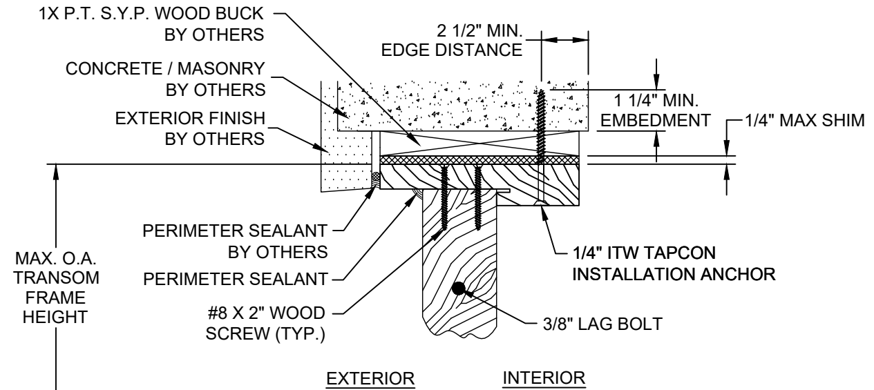
T VERTICAL SECTION GLAZED TRANSOM PANEL AT HEAD CONCRETE / MASONRY SUBSTRATE OUTSWING SHOWN / INSWING OPPOSITE (SEE SHEET 3 SECTION 2 FOR APPROPRIATE TRANSOM PANEL)
