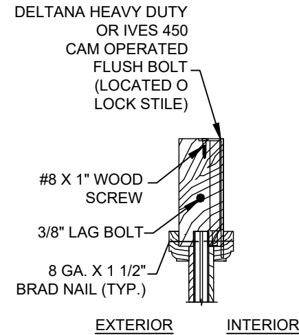
3 3 VERTICAL CROSS SECTION GLAZED 3/4 LITE OVER 2 1/4" WOOD OPAQUE PANEL DOOR, & OPTIONAL SIDELITE PANELS
