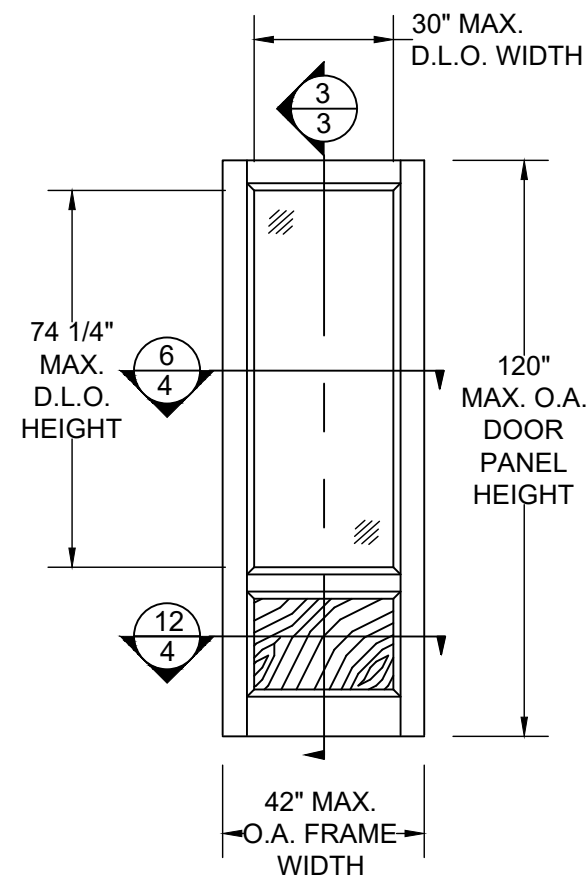
GLAZED 3/4 LITE OVER WOOD PANEL (DOOR & SIDELITE PANELS)
