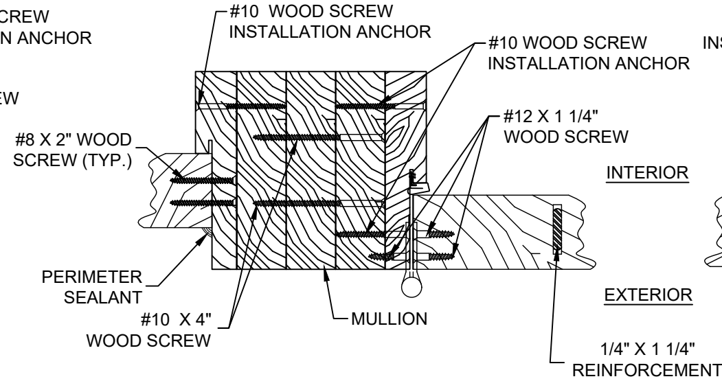
KK HORIZONTAL SECTION GLAZED/OPAQUE SIDELITE PANEL JAMB W/ GLAZED/OPAQUE DOOR PANEL AT MULLION OUTSWING SHOWN / INSWING OPPOSITE (SEE SHEET 4 SECTIONS 10,11 & 12 FOR APPROPRIATE DOOR PANELS & SHEET 4 SECTION 13 & 15 FOR APPROPRIATE SIDELITE PANELS)
