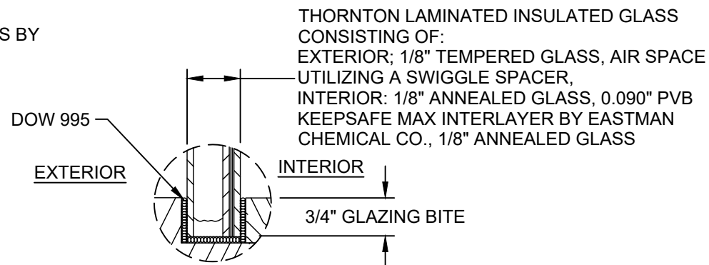
GLAZING DETAIL 2
