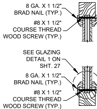
8 3 VERTICAL CROSS SECTION 1 3/4" OPAQUE SASH SET TRANSOM PANELS
