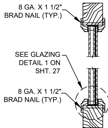
7 3 VERTICAL CROSS SECTION 1 3/4" GLAZED SASH SET TRANSOM PANELS
