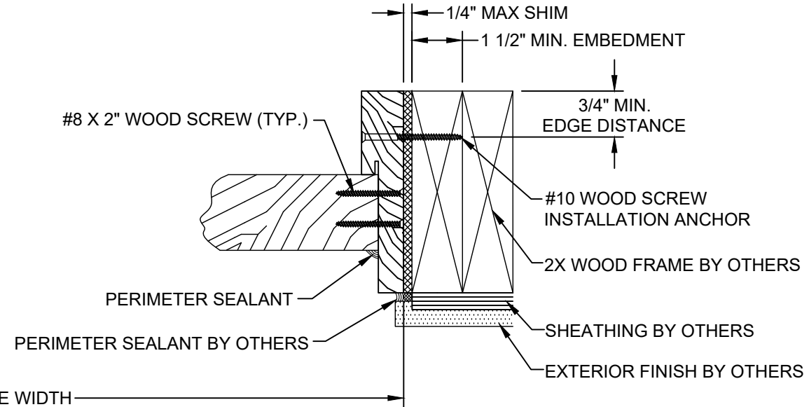
BB HORIZONTAL SECTION GLAZED/OPAQUE SIDELITE / GLAZED TRANSOM PANEL AT JAMB WOOD FRAME SUBSTRATE OUTSWING SHOWN / INSWING OPPOSITE (SEE SHEET 4 SECTIONS 10, 11 & 12 FOR APPROPRIATE SIDELITE PANELS & SHEET 4 SECTION 11 FOR APPROPRIATE TRANSOM PANEL)
