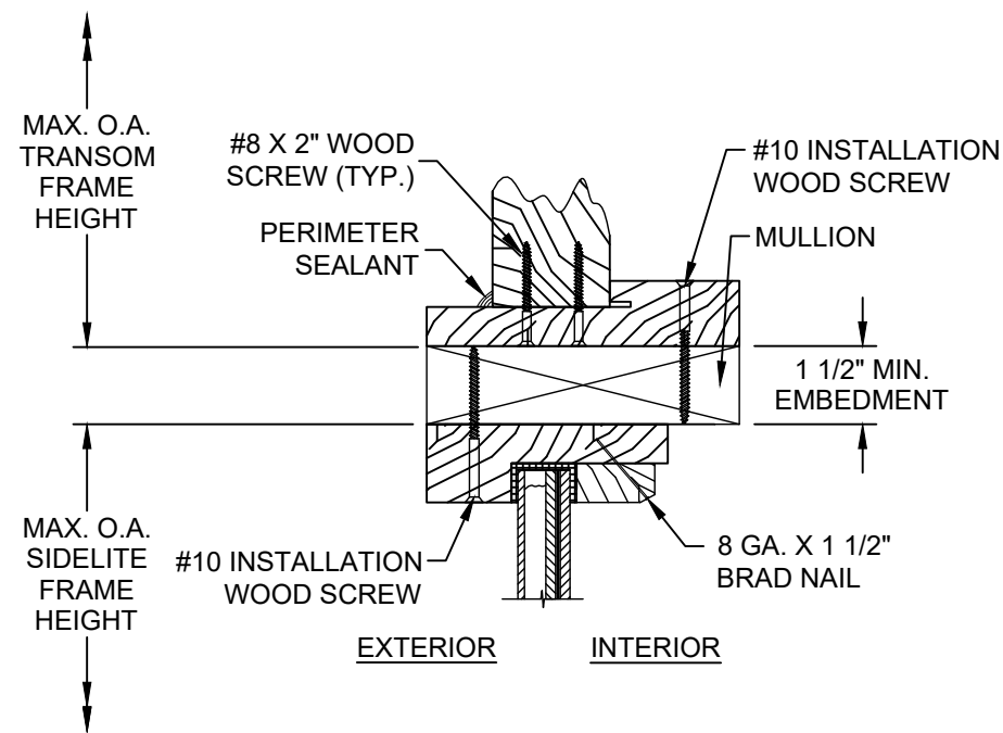
VERTICAL SECTION GLAZED SIDELITE PANEL AT HEAD & GLAZED/OPAQUE TRANSOM SILL AT MULLION OUTSWING SHOWN / INSWING OPPOSITE (SEE SHEET 3 SECTION 5 FOR APPROPRIATE SIDELITE PANEL & SECTIONS 7 & 8 FOR APPROPRIATE TRANSOM PANELS)
