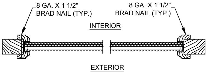
13 4 HORIZONTAL CROSS SECTION 1 3/4" GLAZED SASH SET SIDELITE & TRANSM PANELS
