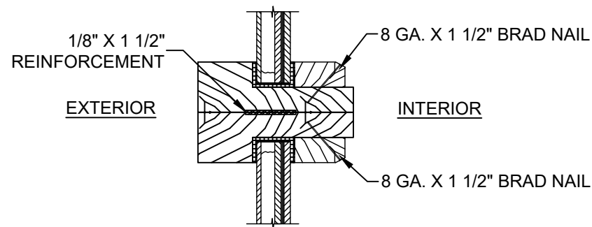
N VERTICAL SECTION GLAZED SIDELITE AT INTERMEDIATE RAIL OUTSWING SHOWN / INSWING OPPOSITE (SEE SHEET 3 SECTION 5 FOR APPROPRIATE SIDELITE PANEL)
