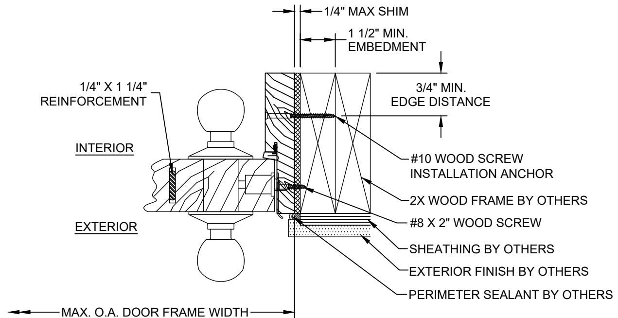
V HORIZONTAL SECTION GLAZED/OPAQUE DOOR PANEL AT LOCK STILE WOOD FRAME SUBSTRATE OUTSWING SHOWN / INSWING OPPOSITE (SEE SHEET 4 SECTIONS 10, 11 & 12 FOR APPROPRIATE DOOR PANELS)
