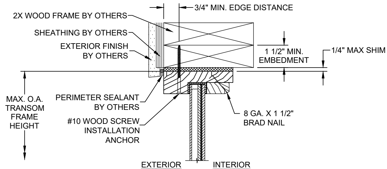
P VERTICAL SECTION GLAZED TRANSOM PANEL AT HEAD WOOD FRAME SUBSTRATE OUTSWING SHOWN / INSWING OPPOSITE (SEE SHEET 3 SECTION 5 FOR APPROPRIATE TRANSOM PANEL)
