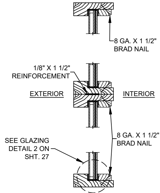
5 3 VERTICAL CROSS SECTION GLAZED DIRECT SET SIDELITE & TRANSOM PANELS
