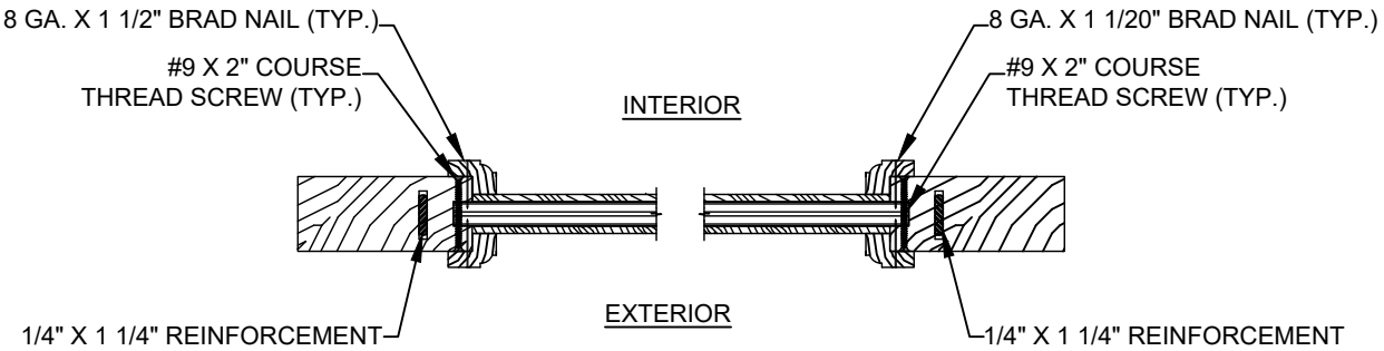
12 4 HORIZONTAL CROSS SECTION 2 1/4" WOOD PANEL UNDER 3/4 LITE GLAZED DOOR & OPTIONAL SIDELITE PANELS
