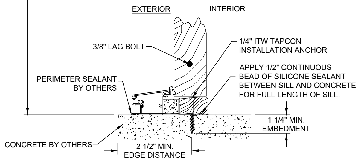
(OPTIONAL A.D.A. THRESHOLD W/ 36" X 96" MAX. O.A. DOOR PANELS @ ±50.0 PSF D.P.) A VERTICAL SECTION GLAZED/OPAQUE DOOR PANEL AT SILL CONCRETE SUBSTRATE INSWING (SEE SHEET 3 SECTIONS 1, 2, 3 & 9 FOR APPROPRIATE DOOR PANELS)
