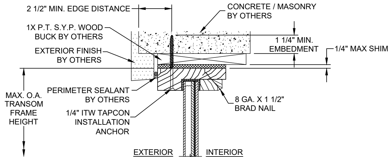
O VERTICAL SECTION GLAZED TRANSOM AT HEAD CONCRETE / MASONRY SUBSTRATE OUTSWING SHOWN / INSWING OPPOSITE (SEE SHEET 3 SECTION 5 FOR APPROPRIATE TRANSOM PANEL)
