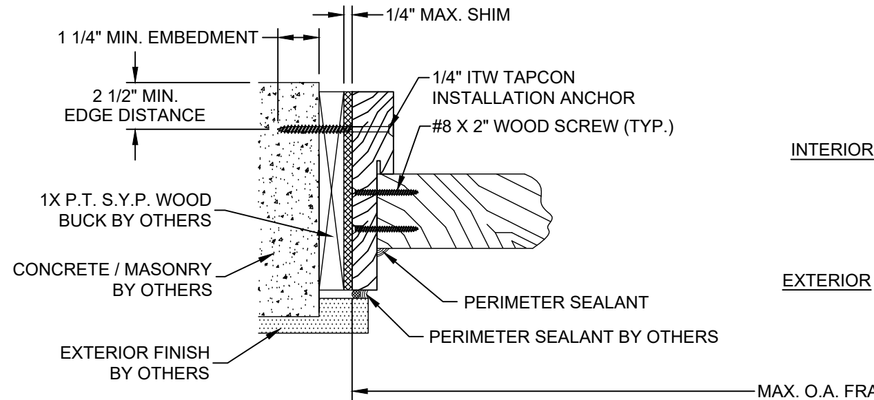
AA HORIZONTAL SECTION GLAZED/OPAQUE SIDELITE / GLAZED TRANSOM PANEL AT JAMB CONCRETE / MASONRY SUBSTRATE OUTSWING SHOWN / INSWING OPPOSITE (SEE SHEET 4 SECTIONS 10, 11 & 12 FOR APPROPRIATE SIDELITE PANELS & SHEET 4 SECTION 11 FOR APPROPRIATE TRANSOM PANEL)
