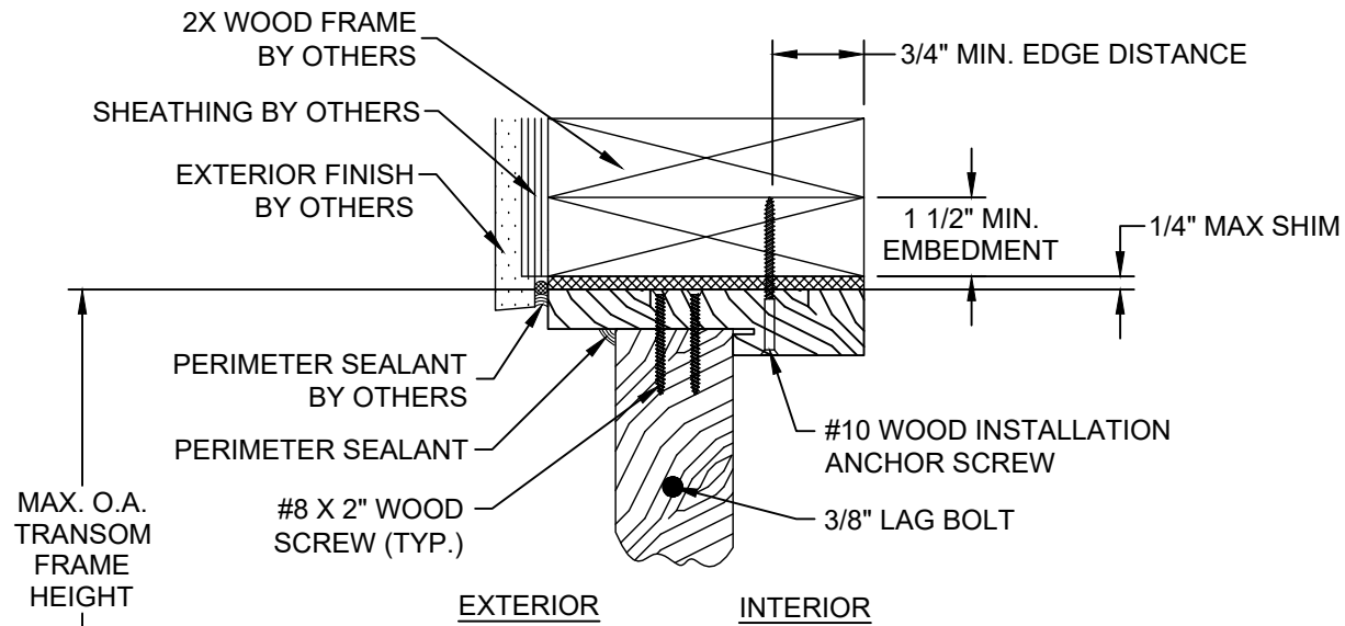
S VERTICAL SECTION GLAZED TRANSOM PANEL AT HEAD WOOD FRAME SUBSTRATE OUTSWING SHOWN / INSWING OPPOSITE (SEE SHEET 3 SECTION 2 FOR APPROPRIATE TRANSOM PANEL)
