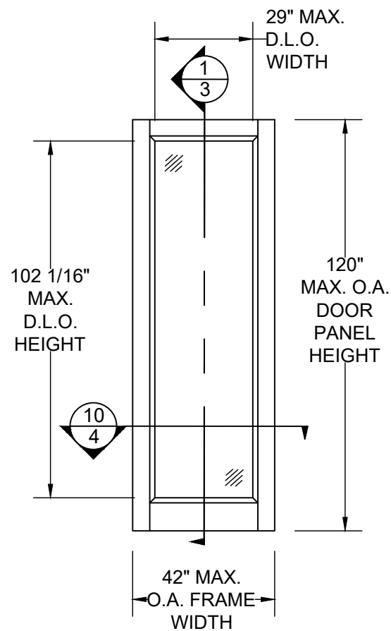
GLAZED FULL LITE PANEL (DOOR & SIDELITE PANELS)
