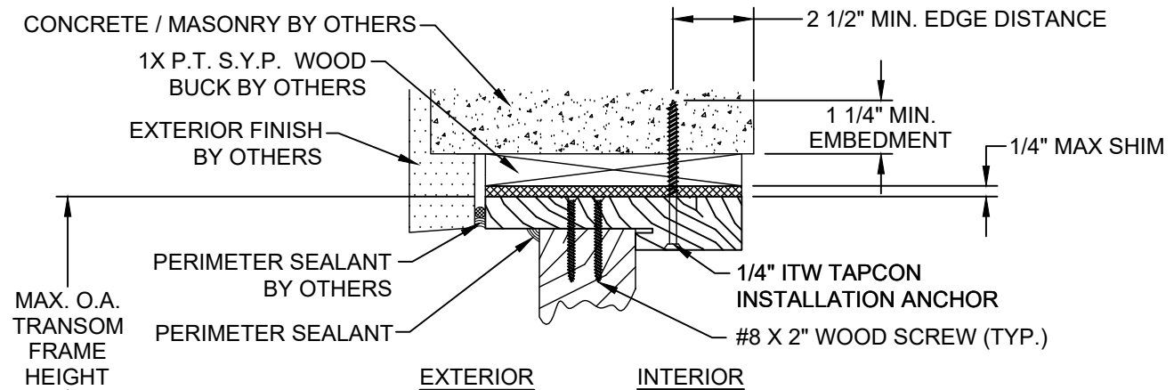
R VERTICAL SECTION GLAZED/OPAQUE TRANSOM PANEL AT HEAD CONCRETE / MASONRY SUBSTRATE OUTSWING SHOWN / INSWING OPPOSITE (SEE SHEET 3 SECTIONS 7 & 8 FOR APPROPRIATE TRANSOM PANELS)
