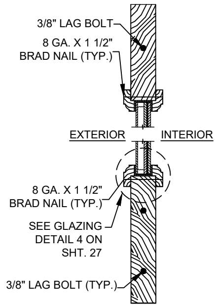
4 3 VERTICAL CROSS SECTION 1 3/4" GLAZED SASH SET SIDELITE PANELS
