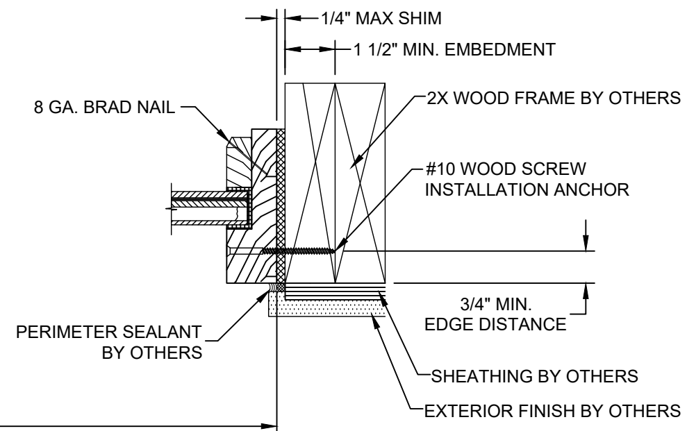
Z HORIZONTAL SECTION GLAZED SIDELITE/TRANSOM PANEL AT JAMB WOOD FRAME SUBSTRATE OUTSWING SHOWN / INSWING OPPOSITE (SEE SHEET 4 SECTION 14 FOR APPROPRIATE SIDELITE & TRANSOM PANELS)
