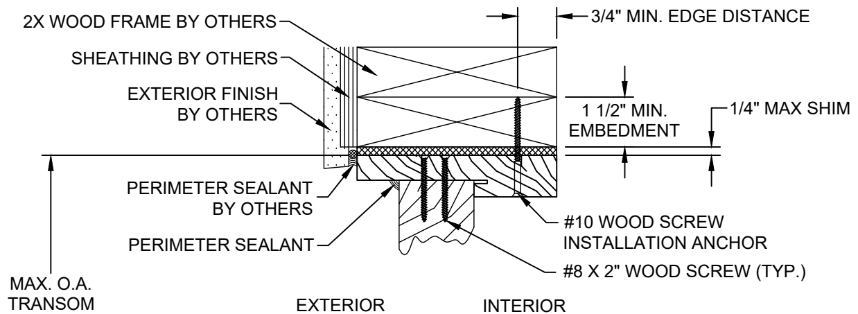
VERTICAL SECTION GLAZED TRANSOM PANEL AT HEAD WOOD FRAME SUBSTRATE OUTSWING SHOWN / INSWING OPPOSITE (SEE SHEET 3 SECTION 7 & 8 FOR APPROPRIATE TRANSOM PANELS)
