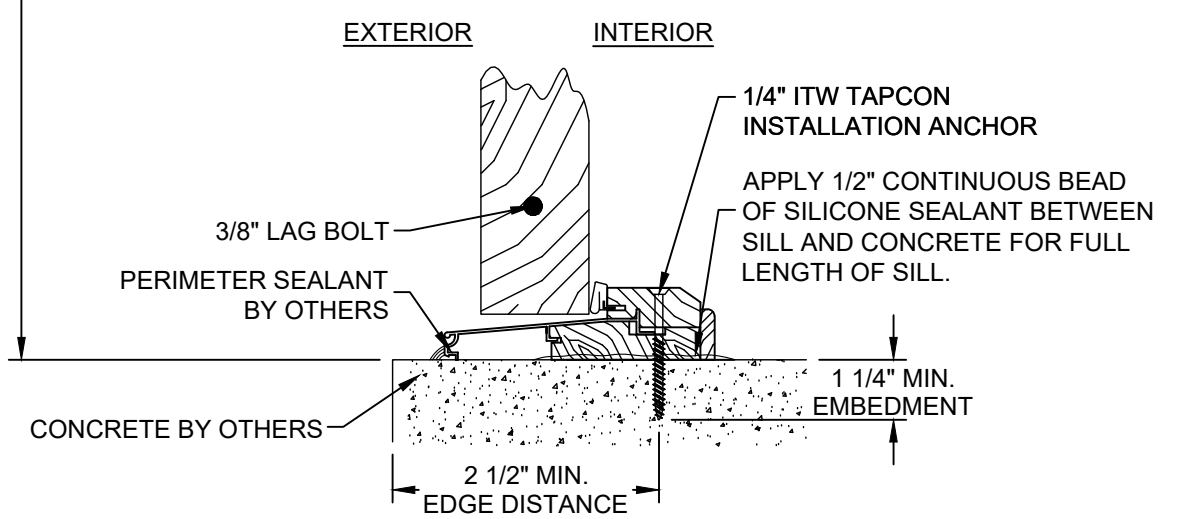
(OPTIONAL A.D.A. THRESHOLD W/ 36" X 96" MAX. O.A. DOOR PANELS @ ±50.0 PSF D.P.) B VERTICAL SECTION GLAZED/OPAQUE DOOR PANEL AT SILL CONCRETE SUBSTRATE OUTSWING (SEE SHEET 3 SECTIONS 1, 2, 3 & 9 FOR APPROPRIATE DOOR PANELS)
