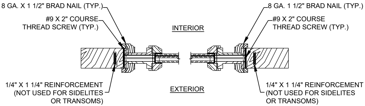
11 4 HORIZONTAL CROSS SECTION 2 1/4" FULL LITE PANEL INSERT DOOR, OPTIONAL SIDELITE & TRANSM PANELS
