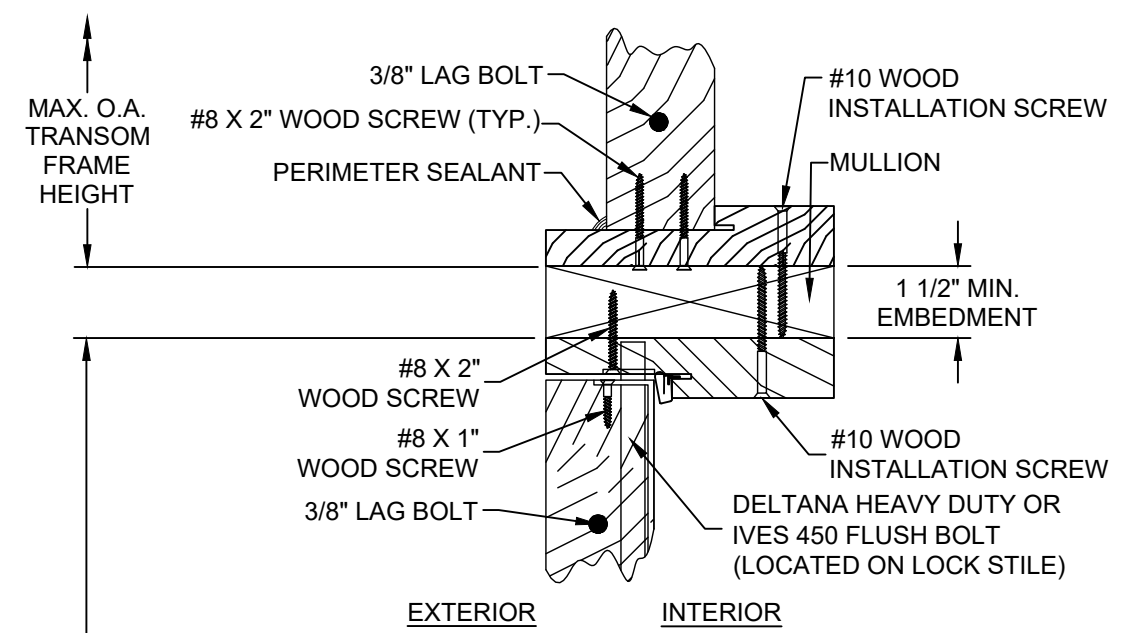
D VERTICAL SECTION GLAZED/OPAQUE DOOR PANEL AT HEAD & GLAZED TRANSOM SILL AT MULLION OUTSWING SHOWN / INSWING OPPOSITE (SEE SHEET 3 SECTIONS 1, 2, 3 & 9 FOR APPROPRIATE DOOR PANELS & SHEET 3 SECTION 2 FOR APPROPRIATE TRANSOM PANEL)
