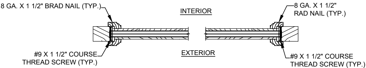
15 4 HORIZONTAL CROSS SECTION 1 3/4" OPAQUE SASH SET SIDELITE & TRANSM PANELS
