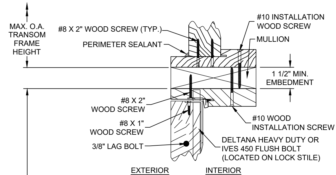
C VERTICAL SECTION GLAZED/OPAQUE DOOR PANEL AT HEAD & GLAZED/OPAQUE TRANSOM SILL AT MULLION OUTSWING SHOWN / INSWING OPPOSITE (SEE SHEET 3 SECTIONS 1, 2, 3 & 9 FOR APPROPRIATE DOOR PANELS & SHEET 3 SECTIONS 7 & 8 FOR APPROPRIATE TRANSOM PANELS)
