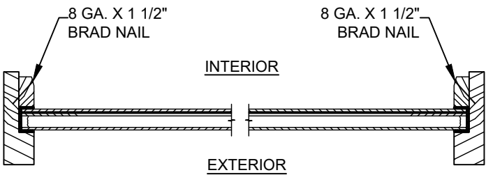
14 4 HORIZONTAL CROSS SECTION GLAZED DIRECT SET SIDELITE & TRANSM PANELS
