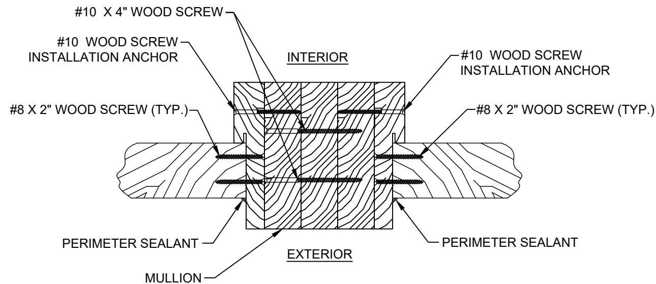
HH HORIZONTAL SECTION GLAZED TRANSOM PANEL JAMBS AT MULLION OUTSWING SHOWN / INSWING OPPOSITE (SEE SHEET 4 SECTION 11 FOR APPROPRIATE TRANSOM PANELS)
