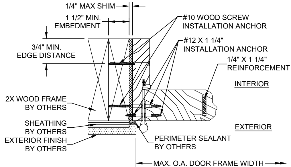
X HORIZONTAL SECTION GLAZED/OPAQUE DOOR PANEL AT HINGED JAMB WOOD FRAME SUBSTRATE OUTSWING SHOWN / INSWING OPPOSITE (SEE SHEET 4 SECTIONS 10, 11 & 12 FOR APPROPRIATE DOOR PANELS)
