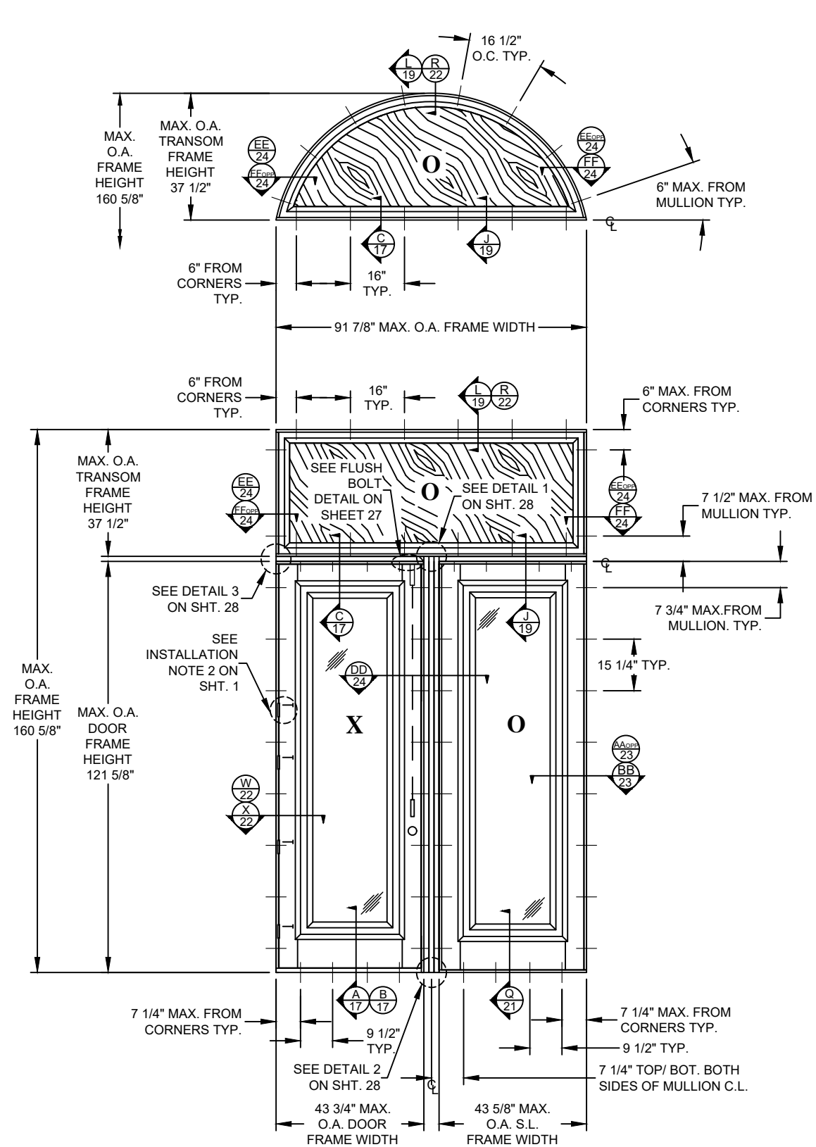
ELEVATION & ANCHOR LAYOUT GLAZED/OPAQUE SINGLE DOOR W/ GLAZED/OPAQUE SIDELITE & OPAQUE SASH SET SQUARE/RADIUS TOP TRANSOM INSWING / OUTSWING EXTERIOR VIEW \frac{O}{XO}
