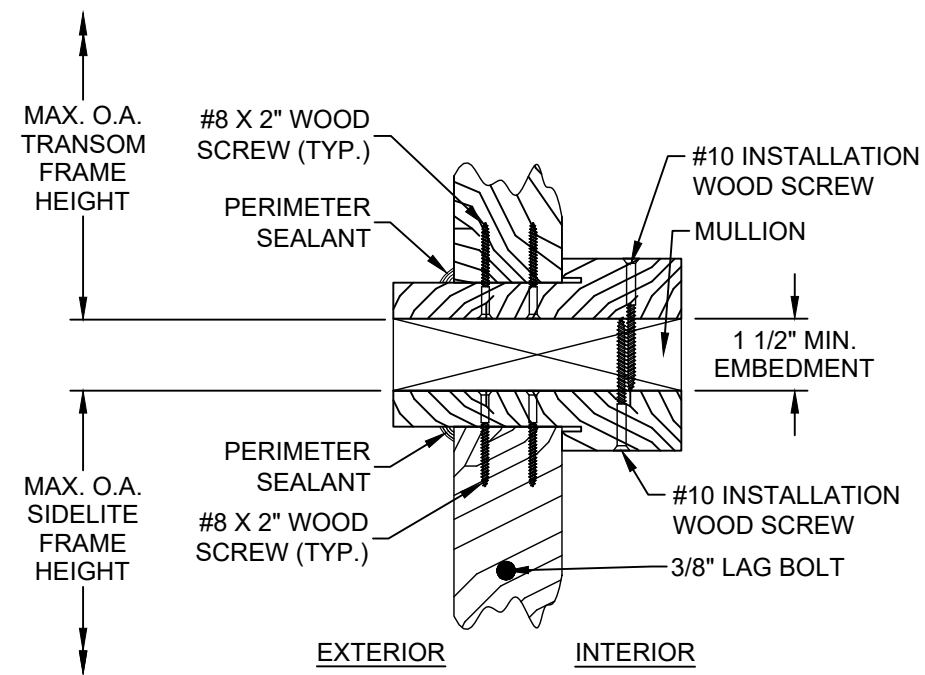
VERTICAL SECTION GLAZED SIDELITE PANEL AT HEAD & GLAZED/OPAQUE TRANSOM SILL AT MULLION OUTSWING SHOWN / INSWING OPPOSITE (SEE SHEET 3 SECTIONS 1, 2, 3, 4 & 6 FOR APPROPRIATE SIDELITE PANELS & SECTIONS 7 & 8 FOR APPROPRIATE TRANSOM PANELS)
