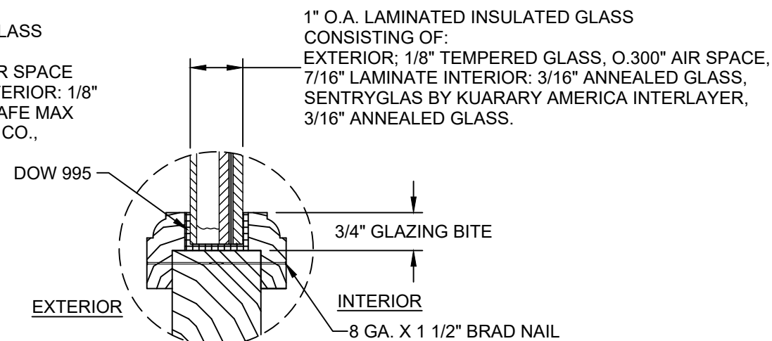
GLAZING DETAIL 4
