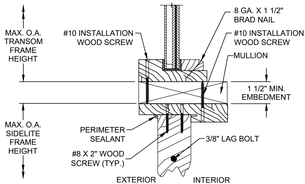
VERTICAL SECTION GLAZED/OPAQUE SIDELITE PANEL AT HEAD & GLAZED TRANSOM SILL AT MULLION OUTSWING SHOWN / INSWING OPPOSITE (SEE SHEET 3 SECTIONS 1, 2, 3, 4, & 6 FOR APPROPRIATE SIDELITE PANELS & SECTION 5 FOR APPROPRIATE TRANSOM PANEL)
