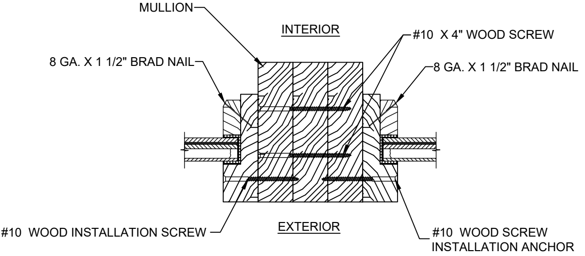
NN HORIZONTAL SECTION GLAZED TRANSOM PANEL JAMBS AT MULLION OUTSWING SHOWN / INSWING OPPOSITE (SEE SHEET 4 SECTION 14 FOR APPROPRIATE TRANSOM PANELS)
