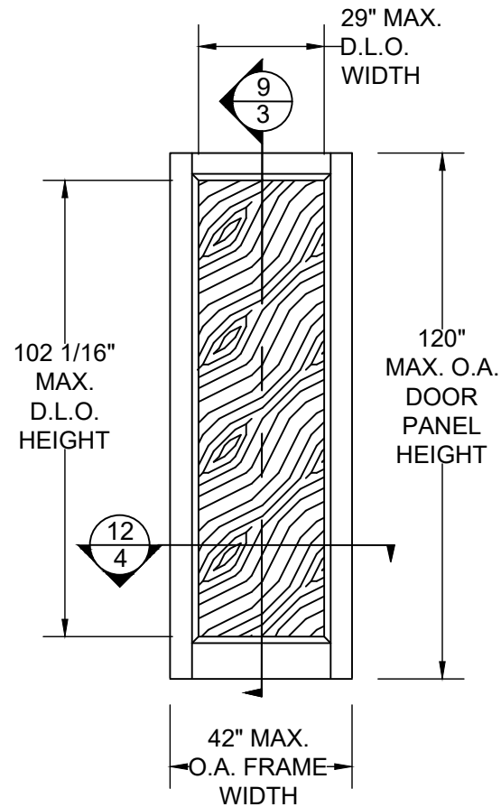
OPAQUE FULL LITE (DOOR & SIDELITE PANELS)
