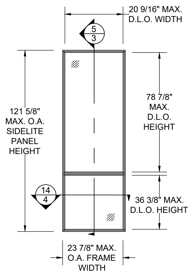
GLAZED DIRECT SET PANEL (SIDELITE & TRANSOM PANELS)
